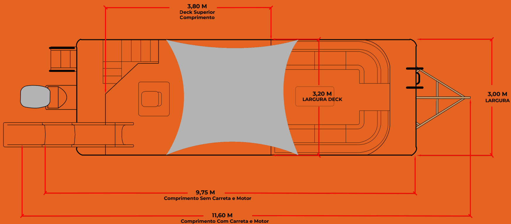
AURORA 900UP VISTA SUPERIOR
